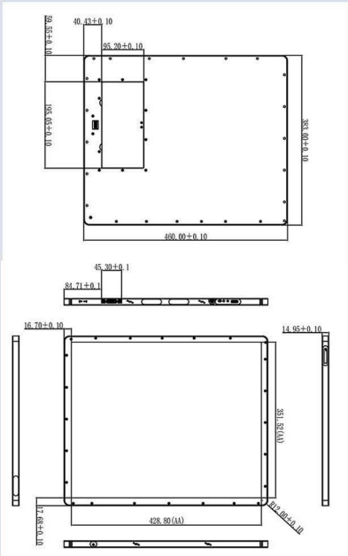
MX-FPD4343 SIZE
